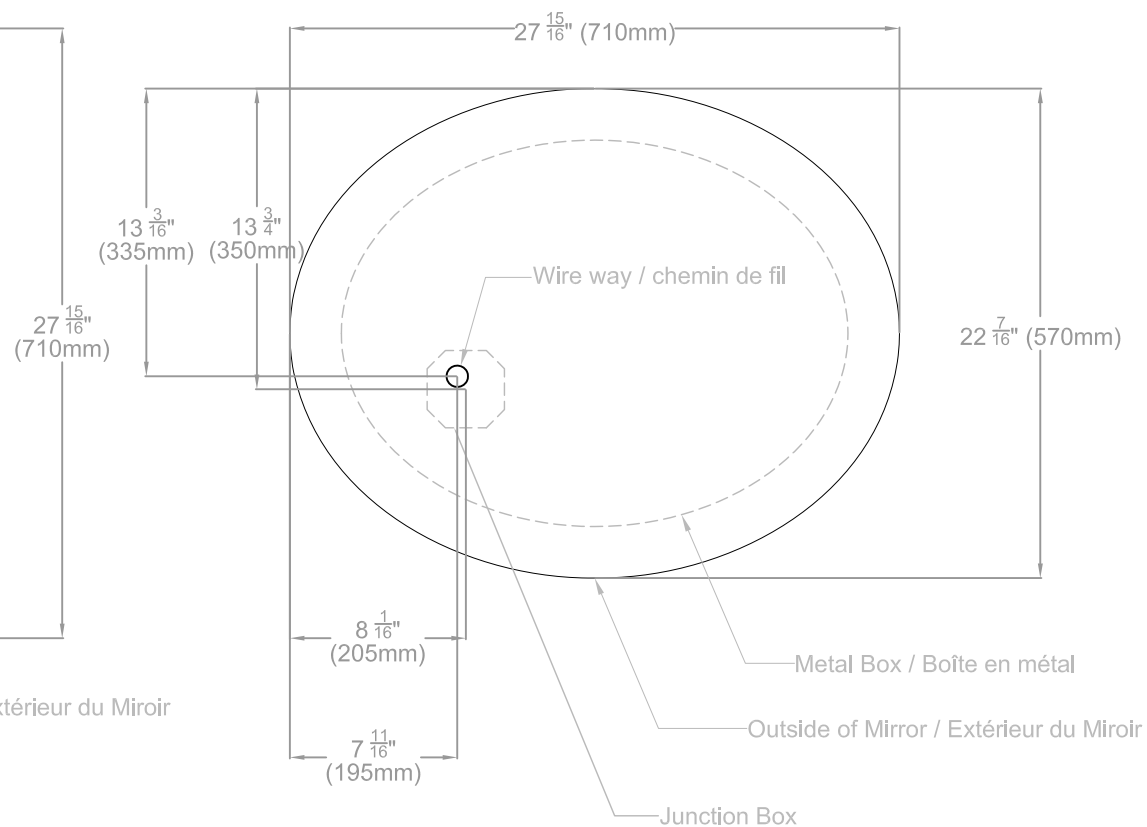
Horizontal mounting / Montage Horizontal
